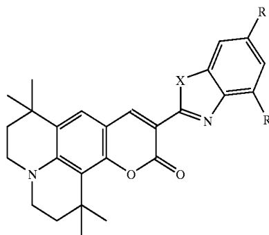
FD 27 R = R' = H, X = O FD 28 R = H, R' = Me, X = O FD 29 R = Me, R' = H, X = O FD 30 R = Me, R' = Me, X = O FD 31 R = H, R' = t-Bu, X = O FD 32 R = t-Bu, R' = H, X = O FD 33 R = R' = t-Bu, X = O FD 34 R = R' = H, X = S FD 35 R = H, R' = Me, X = S FD 36 R = Me, R' = H, X = S FD 37 R = Me, R' = Me, X = S FD 38 R = H, R' = t-Bu, X = S FD 39 R = t-Bu, R' = H, X = S FD 40 R = R' = t-Bu, X = S
