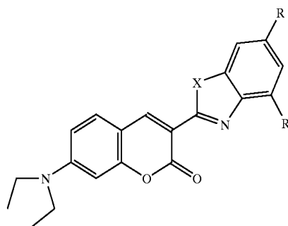
FD 13 R = R' = H, X = O FD 14 R = H, R' = Me, X = O FD 15 R = Me, R' = H, X = O FD 16 R = Me, R' = Me, X = O FD 17 R = H, R' = t-Bu, X = O FD 18 R = t-Bu, R' = H, X = O FD 19 R = R' = t-Bu, X = O FD 20 R = R' = H, X = S FD 21 R = H, R' = Me, X = S FD 22 R = Me, R' = H, X = S FD 23 R = Me, R' = Me, X = S FD 24 R = H, R' = t-Bu, X = S FD 25 R = t-Bu, R' = H, X = S FD 26 R = R' = t-Bu, X = S
