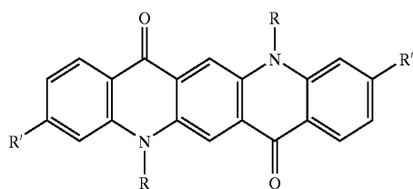
FD 8 R = R' = H FD 9 R = Me, R' = H FD 10 R = Pr-i, R' = H FD 11 R = Me, R' = F FD 12 R = phenyl, R' = H
